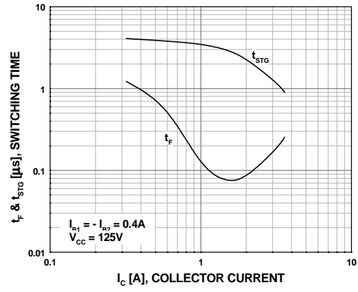
Figure 8. Switching Time
