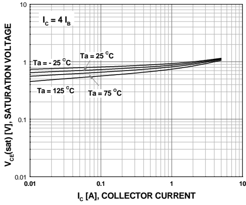
Figure 7. Saturation Voltage (O-Grade)
